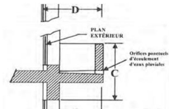
Figure 2.5 : Garde-corps
